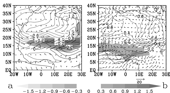
Figure 2. a) First SVD mode of anomalous MSLP [hPa] (contours) and rainfall [ \text{mm day}^{-1} ] (shaded) for the 10 ensemble integrations with prescribed observed SST from 1940–2002. The patterns are normalized to one standard deviation of the PCs. The arrows are the regression of the moisture flux at 925 hPa [ (\text{kg}\cdot\text{m}) (\text{kg}\cdot\text{s})^{-1} ] onto the normalized PC of the MSLP pattern. b) As a but now for the NCEP/NCAR reanalysis and CMAP data for 1979–2004. The explained total squared covariance in a and b are respectively 51% and 49%. The correlations of the PCs are 0.78 and 0.68.
