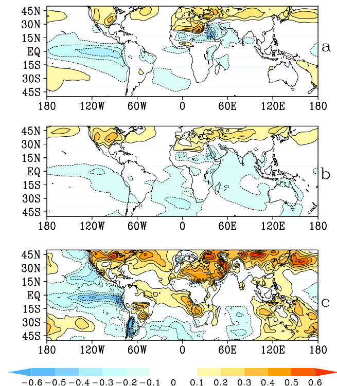
Figure 3. a) Regression of SAT onto the PC of the MSLP pattern of the SVD mode for the forced SST integrations. b) As a but with a 10-year running mean applied. c) As a but now for the NCEP/NCAR reanalysis and CMAP data. The covariances are normalized by the variances of the PCs. The contour interval is 0.1 K. For the SST forced runs all responses larger than 0.1 K are significant according to the 99% threshold of a t-test. Due to the shortness of the NCEP/NCAR and CMAP data the results are only significant according to the 80% threshold.
