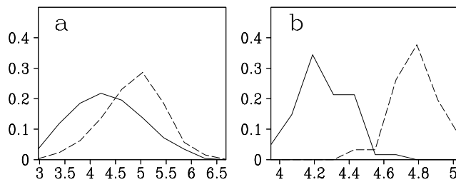
Figure 5. a) Probability density function of JAS rainfall [ \text{mm day}^{-1} ] for the region 10^{\circ}\text{N} – 20^{\circ}\text{N} , 10^{\circ}\text{W} – 30^{\circ}\text{E} . Solid curve: 1950–1980. Dashed curve: 2050–2080 b) As a but 30-year averaged.
