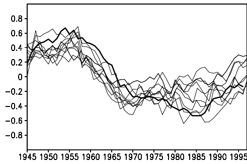
Figure 1. Anomalous rainfall [ \text{mm day}^{-1} ] during JAS for the Sahel region 10^{\circ}\text{N} – 20^{\circ}\text{N} , 10^{\circ}\text{W} – 30^{\circ}\text{E} . Thin lines: Individual model runs. Thick line: Observations. A 10-yr running mean is applied.
